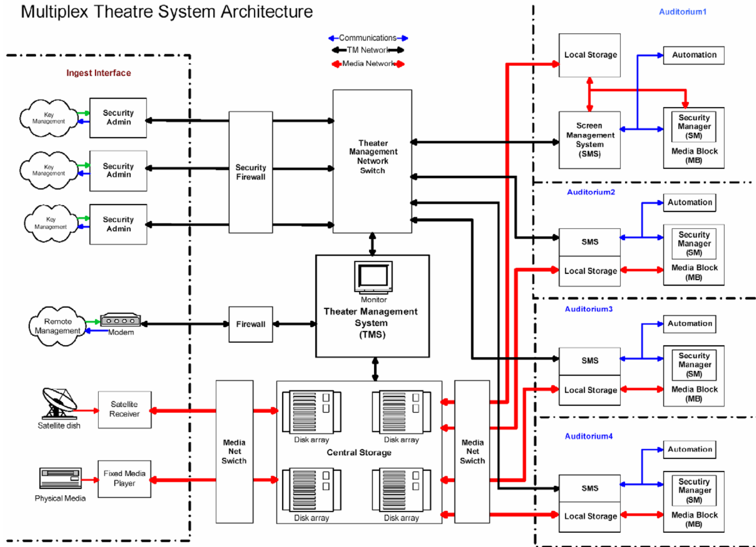
Figure 13: Multiplex Theatre System Architecture
